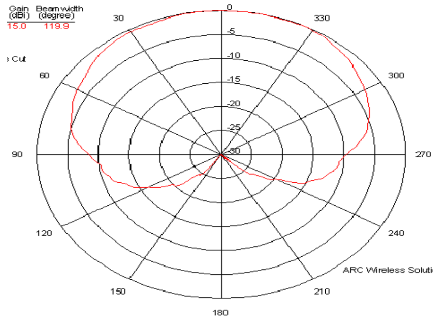
RF Patterns Horizontal Cut
