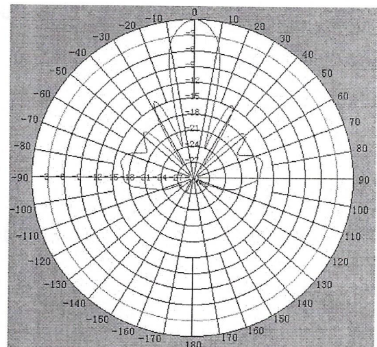
E Plane Radiation Pattern
